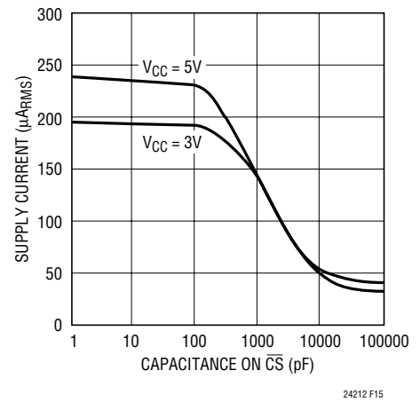
Figure 15. \overline{CS} Capacitance vs Supply Current
